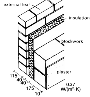
④ Cavity walling 0.37 W/(m 2 ·K)
